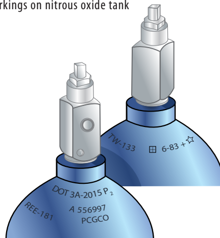
Figure 3. Markings on nitrous oxide tank
